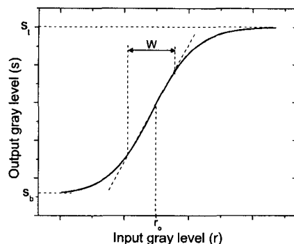
Figure 3.14: Sigmoidal function response of the LC-SLM when contrast = 255 and brightness B > 50 .
