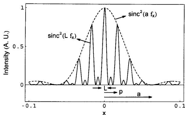
Figure 3.19: Diffraction pattern simulation of LC panel in x -direction.
