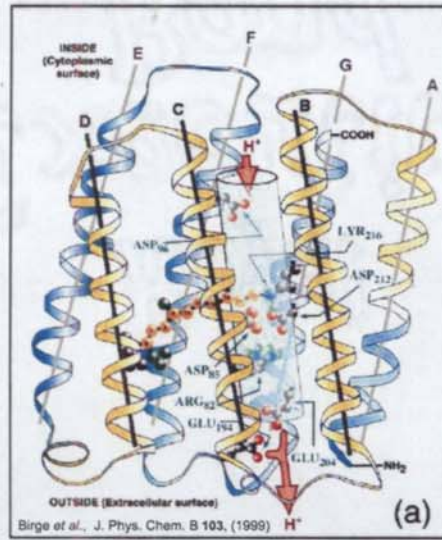
Figure 1.4: Molecular structure of bacteriorhodopsin.
