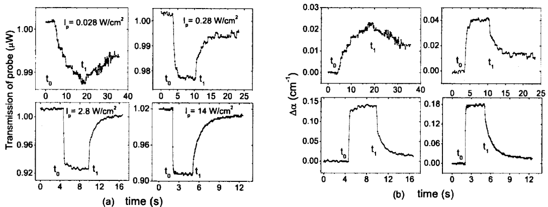
Figure 2.5: (a) Probe beam transmission ( \lambda_s = 633 nm ) through undoped \text{BaTiO}_3 crystal when illuminated by pump at 514 nm at different intensities and, (b) corresponding LIA change.
