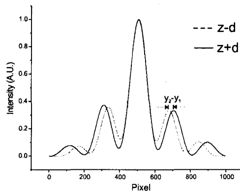
Figure 3.22: Intensity line profile of a diffraction pattern along y -direction, recorded at two different planes that are 10 mm apart.
