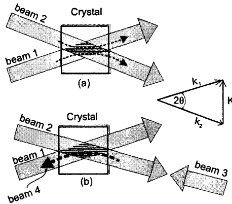
Figure 1.3: Transmission geometry of wave mixing in PR crystal. (a) Two-wave mixing and (b) generation of phase conjugate beam in four-wave mixing.
