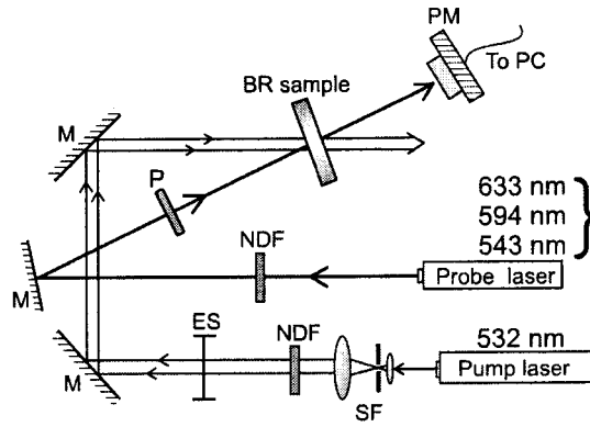
Figure 5.9: Experimental layout for optical switching using pump-probe method. SF, spatial filter with beam expander; P, polarizer; PM, power meter; M, mirror; ES, electronic shutter; NDF, neutral density filter.
