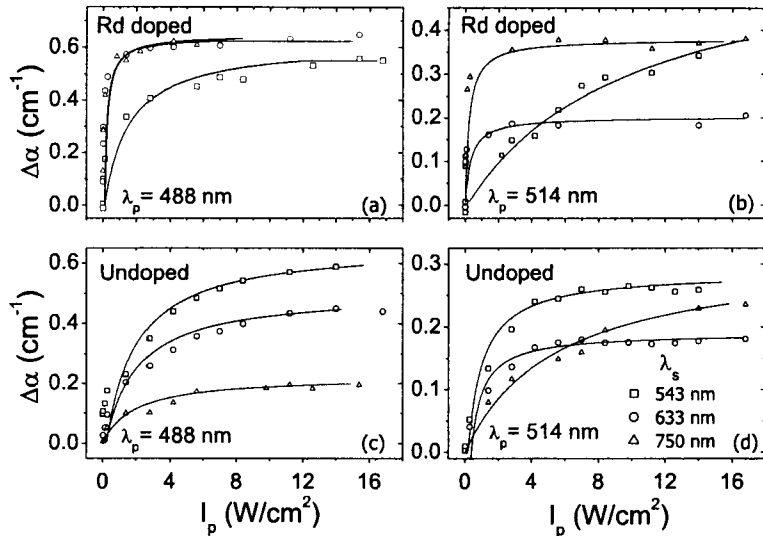
Figure 2.7: Steady-state light-induced absorption change \Delta\alpha versus pump beam intensity at different probe wavelengths. (a)–(b) for Rh-doped and (c)–(d) for undoped \text{BaTiO}_3 crystal.
