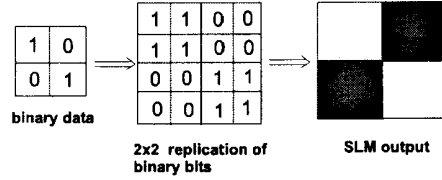
Figure 4.11: Representation of binary data on SLM using 2 \times 2 replication of original bits.
