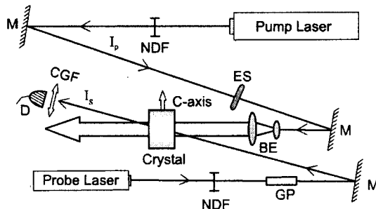
Figure 2.4: Schematic of the experimental setup: M's, mirrors; NDF, neutral density filter; ES, electro-mechanical shutter; GP, Glan laser polarizer; D, detector; BE, beam expander; CGF, colour glass filter; I_p , pump beam; I_s , probe beam.
