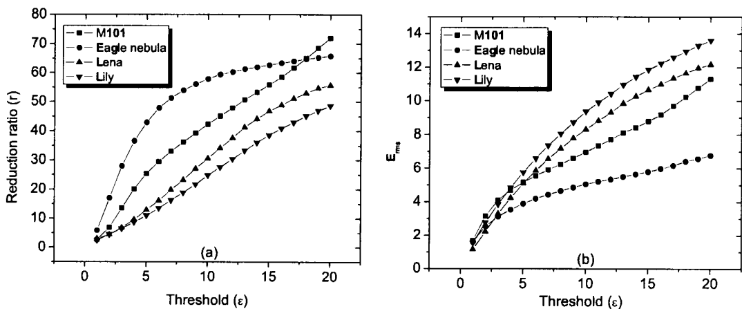
Figure 4.5: The variation of (a) reduction ratio r and (b) root-mean-square error E_{\text{rms}} with threshold \varepsilon .
