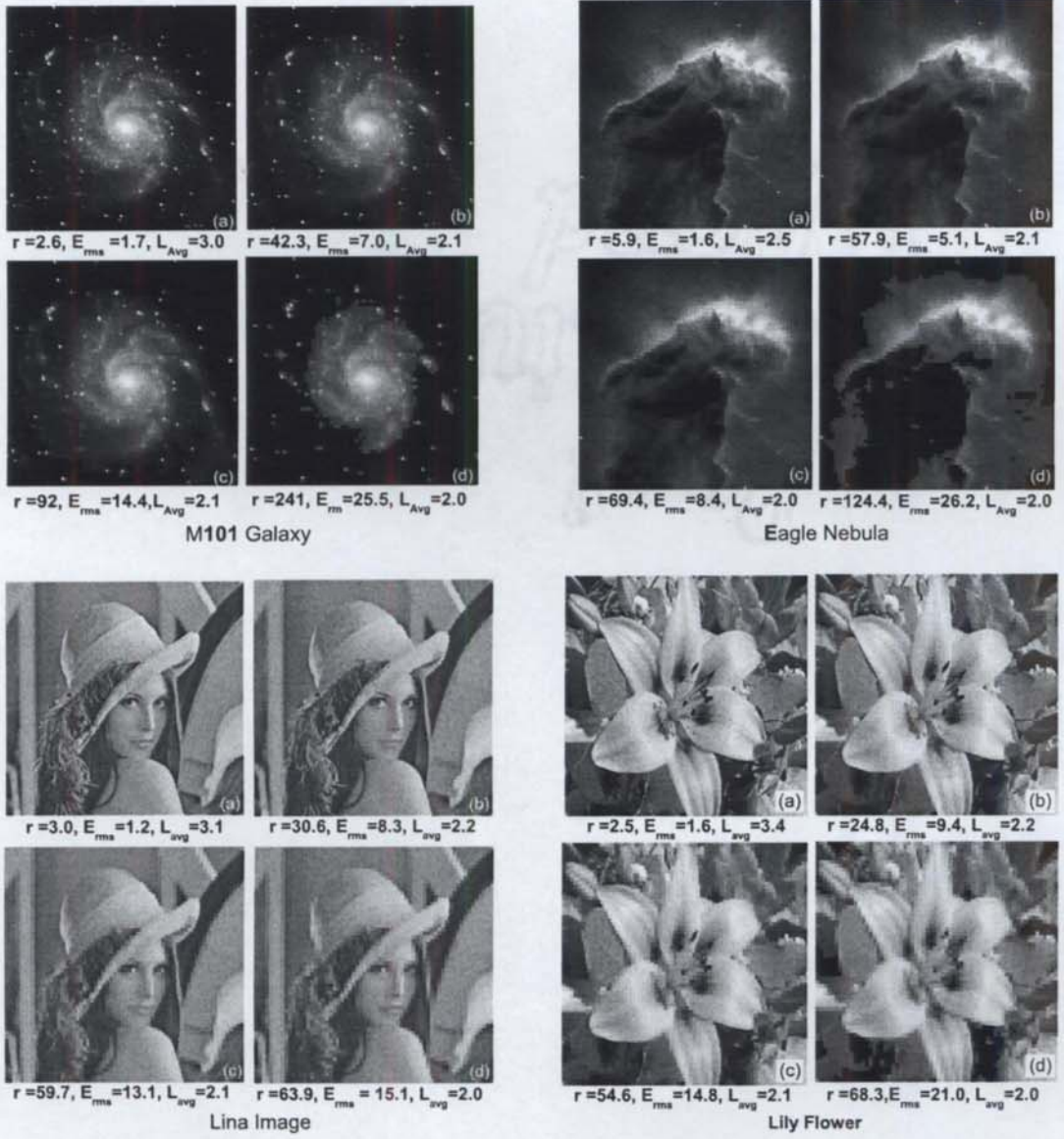
Figure 4.4: The effect of threshold \varepsilon on r , E_{rms} , L_{Avg} (bits/pixel) and the visual image quality of four representative images. (a) \varepsilon = 1 , (b) \varepsilon = 10 , (c) \varepsilon = 25 and (d) \varepsilon = 50 .
