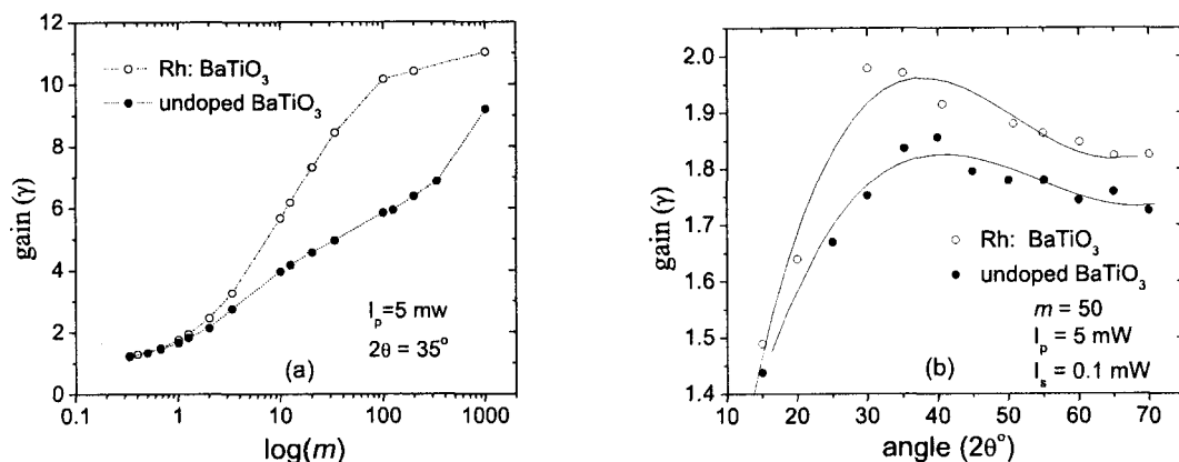
Figure 2.12: (a) Plot of gain vs intensity ratio m (b) gain vs beam-crossing angle measured at 488 nm.
