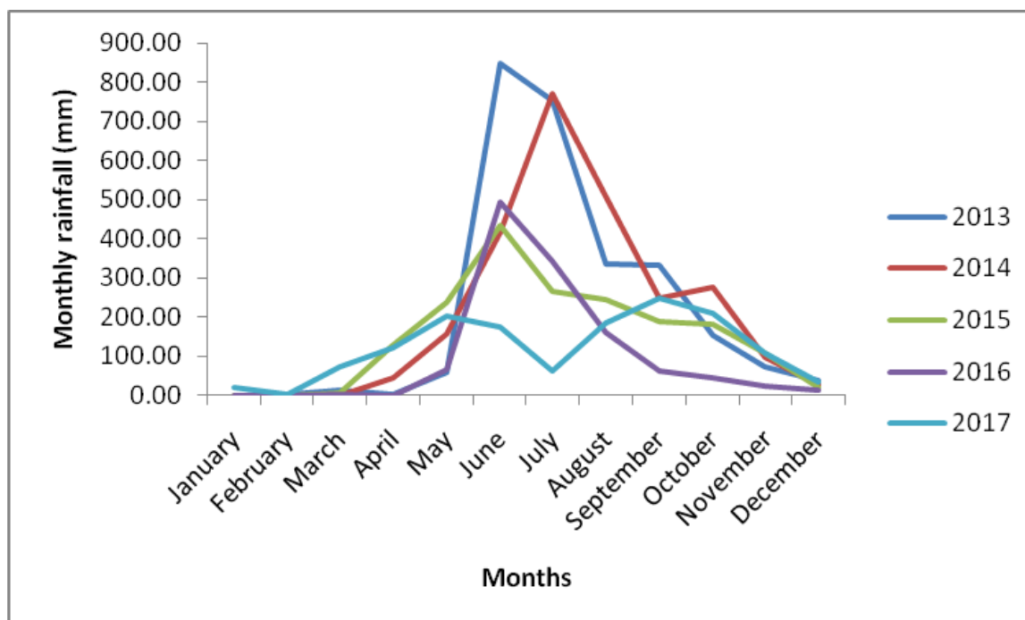
Fig. 03. Mean monthly rainfall over the years (Agricultural Research Station, Anakayam)
