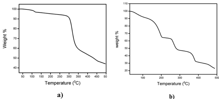
Fig.11. TG curves of a) [Ni(HL) 2 Cl 2 ] and b) [Cd(HL) 2 Cl 2 ]
