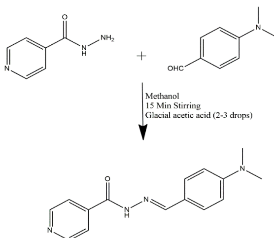
Scheme 1. Synthesis of 4-[N,N-(dimethyl)amino]benzaldehyde isonicotinoylhydrazone (HL)
