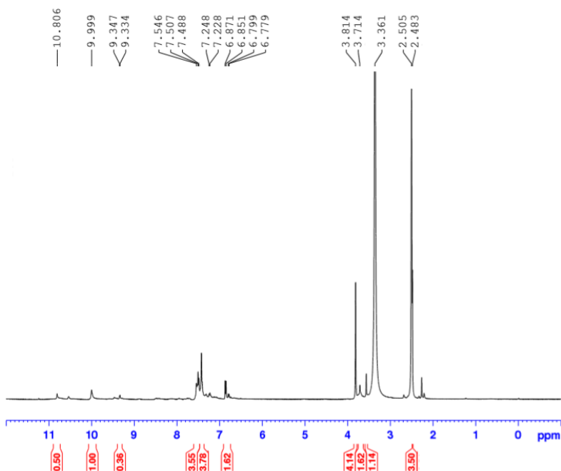
Fig.8. ^1\text{H} NMR spectrum of Zn(II) complex
