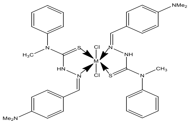
Fig.11. Proposed structure of the complexes,
