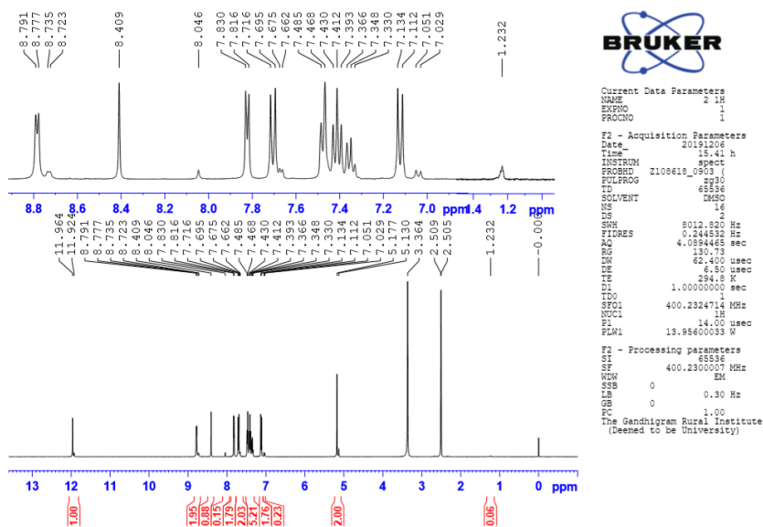
Fig.10. ^1\text{H} NMR Spectrum of [\text{Zn}(\text{HL})_2\text{Cl}_2]
