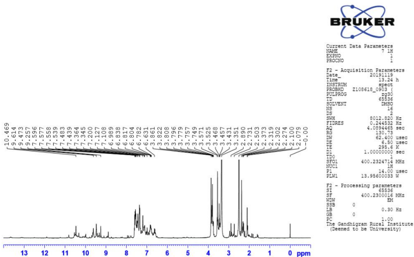
Fig.9. ^1\text{H} NMR spectrum of Cd(II) complex
