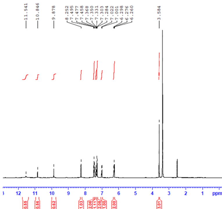
Fig.7. ^1\text{H} NMR spectrum of HL
