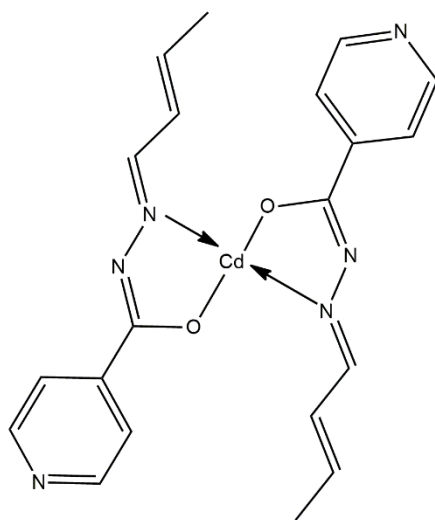
Fig.14. Proposed structure of the complex, [Cd(L)_2]
