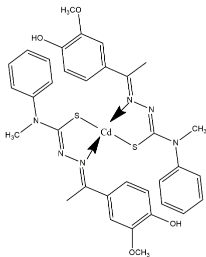
Fig.15. Proposed structure of the complex, [Cd(L)_2]
